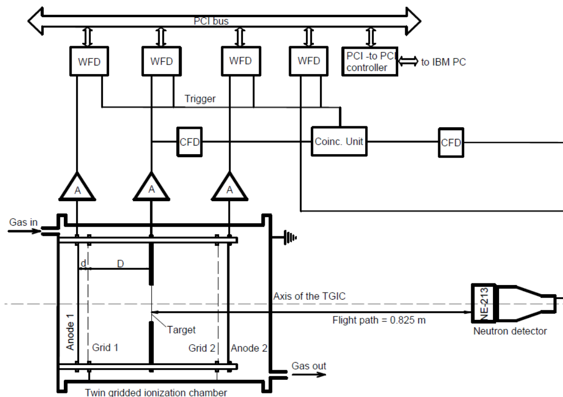
Fig. 1 Sketch of the experimental setup for PFN investigation.
